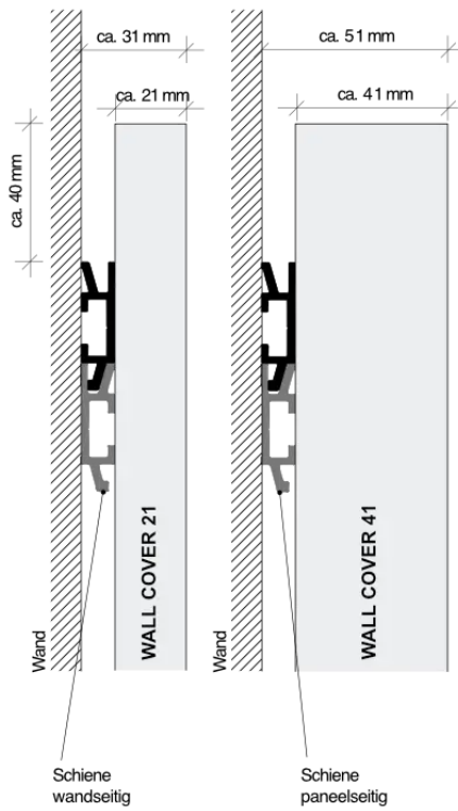
Schienenmontage Rail mounted
