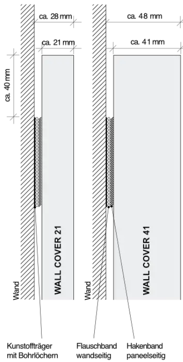
Klettmontage Wand Hook-and-loop mounting walls
