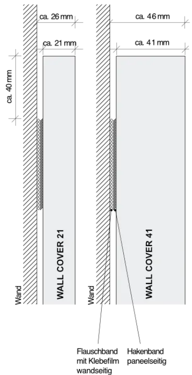
Klettmontage Glas Hook-and-loop mounting glass
